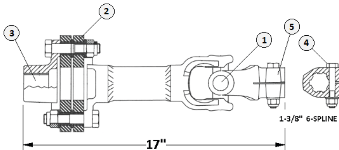
180003 - Complete Connector Shaft for (10-Ft. Cutter)
