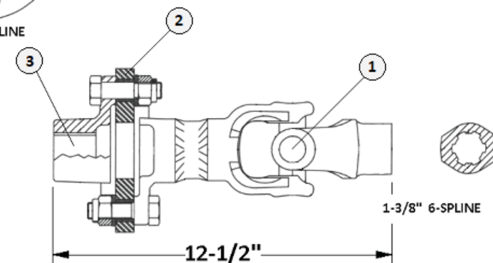
180002 - Complete Connector Shaft for (8-Ft. Cutter)
